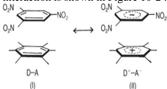
Fig. 10-2. Resonance in a donor-acceptor complex of trinitrobenzene (acceptor, top) and hexamethylbenzene (donor, bottom).
