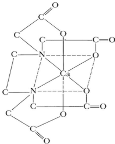
Fig. 10-1. Calcium ions sequestered by ethylenediaminetetraacetic acid.
