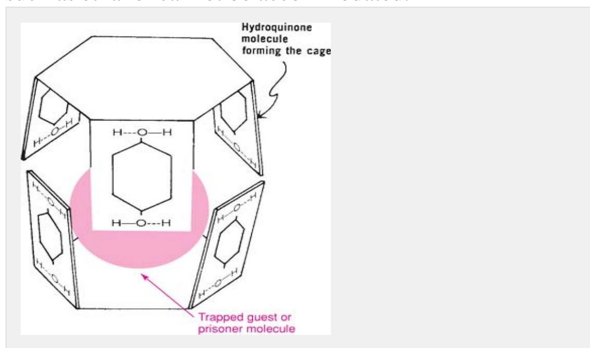
Fig. 10-4. Cagelike structure formed through hydrogen bonding of hydroquinone molecules. Small molecules such as methanol are trapped in the cages to form the clathrate
